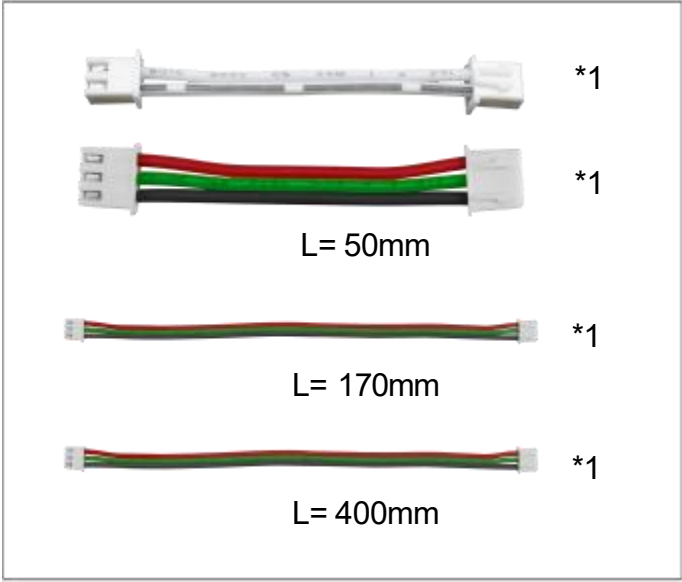
Connection piece*4
